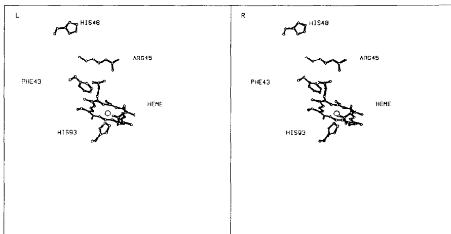
Fig. 6. Myoglobin. Stereodrawing of selected parts of sperm whale myoglobin. Details of the molecular structure of the region His-48 to the heme group. Ru is coordinated to His-48 N ε [67] which is the atom next to the "H" of the His-48 label. The coordinates are taken from the Brookhaven Data Bank, file 1MBO [75].
