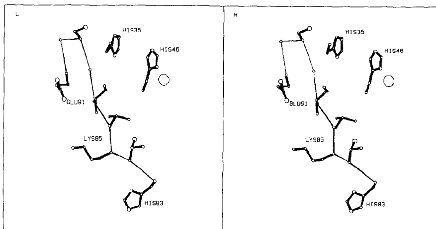
Fig. 3. Azurin. Stereodrawing of the His-83 to Glu-91 peptide strand together with the side-chains of His-35, the copper ligand His-46 and the copper atom (large circle). The data are taken from the same source as mentioned in the legend to Fig. 2.
